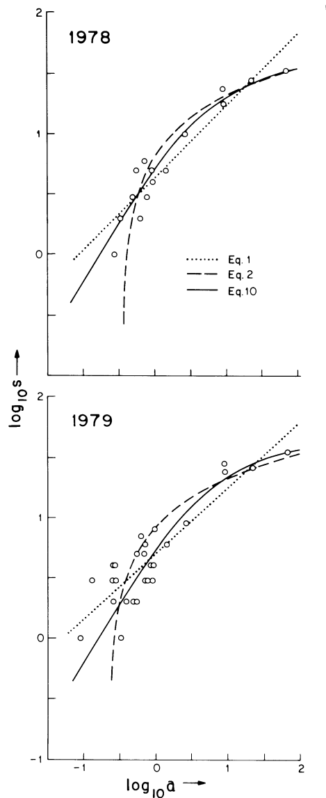
FIG. 5. Comparison of observed values of s with those calculated from the power function of Eq. 1, the exponential relation of Eq. 2, and the expected species-area function \bar{s} derived from the hypothesis of random placement (Eq. 10). The parameter pairs ( c , z ) and ( G , \kappa ) are as in Table 3.
