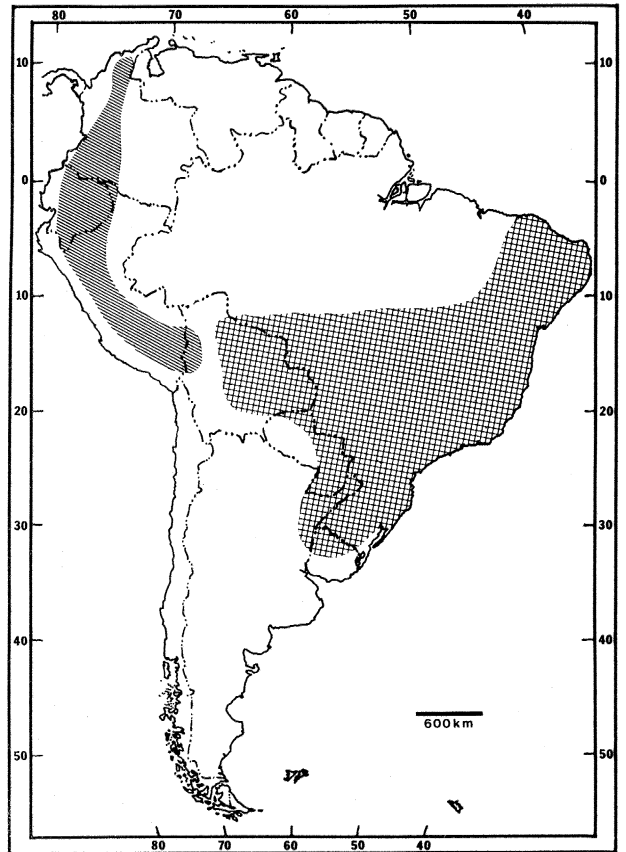
FIG. 3. Distribution of Vampyrops lineatus (principally after Koopman, 1983). Subspecies are V. l. lineatus (crosshatch) and V. l. nigellus (diagonal).
