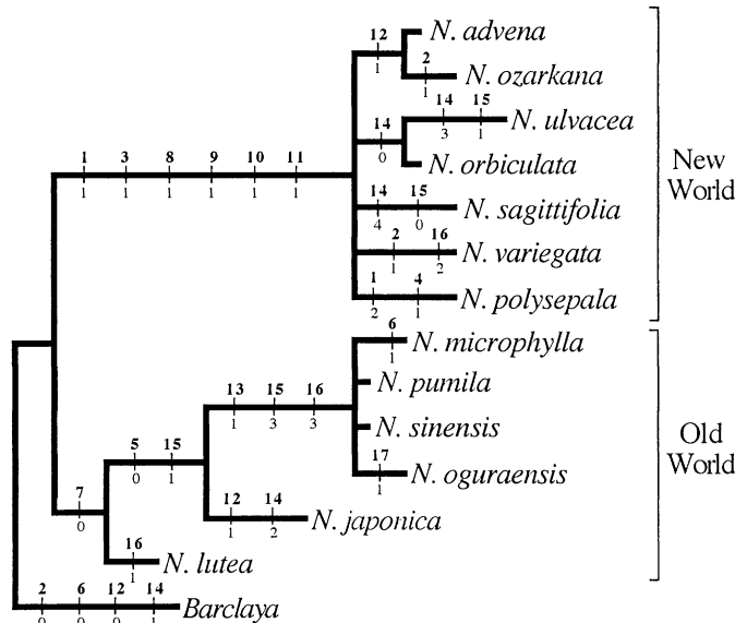
Fig. 1. One of 190 most parsimonious cladograms from a cladistic analysis of 17 morphological characters (length = 32, CI = 0.84, RI = 0.91) showing distribution of characteristics. Character numbers (above the branch) and states (below the branch) correspond to those in Table 1.
