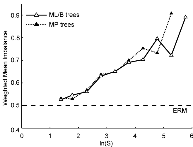
FIGURE 2. The weighted mean imbalance of empirical trees plotted as a function of the natural log of the node size ( S ). The dashed line at 0.5 indicates the imbalance expected under the ERM model. One hundred and twenty-four trees reconstructed using maximum parsimony (MP) are indicated by the dotted line with black triangles and 107 trees reconstructed by maximum likelihood or Bayesian methods (ML/B) are represented by the solid line and white triangles.
