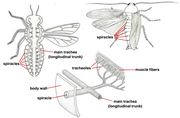
Generalized layout of ventilatory system
