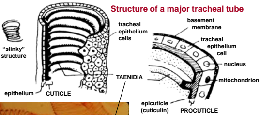
Structure of a major tracheal tube
