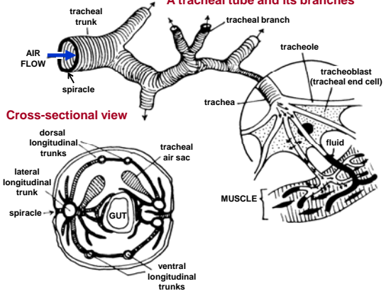
A tracheal tube and its branches
